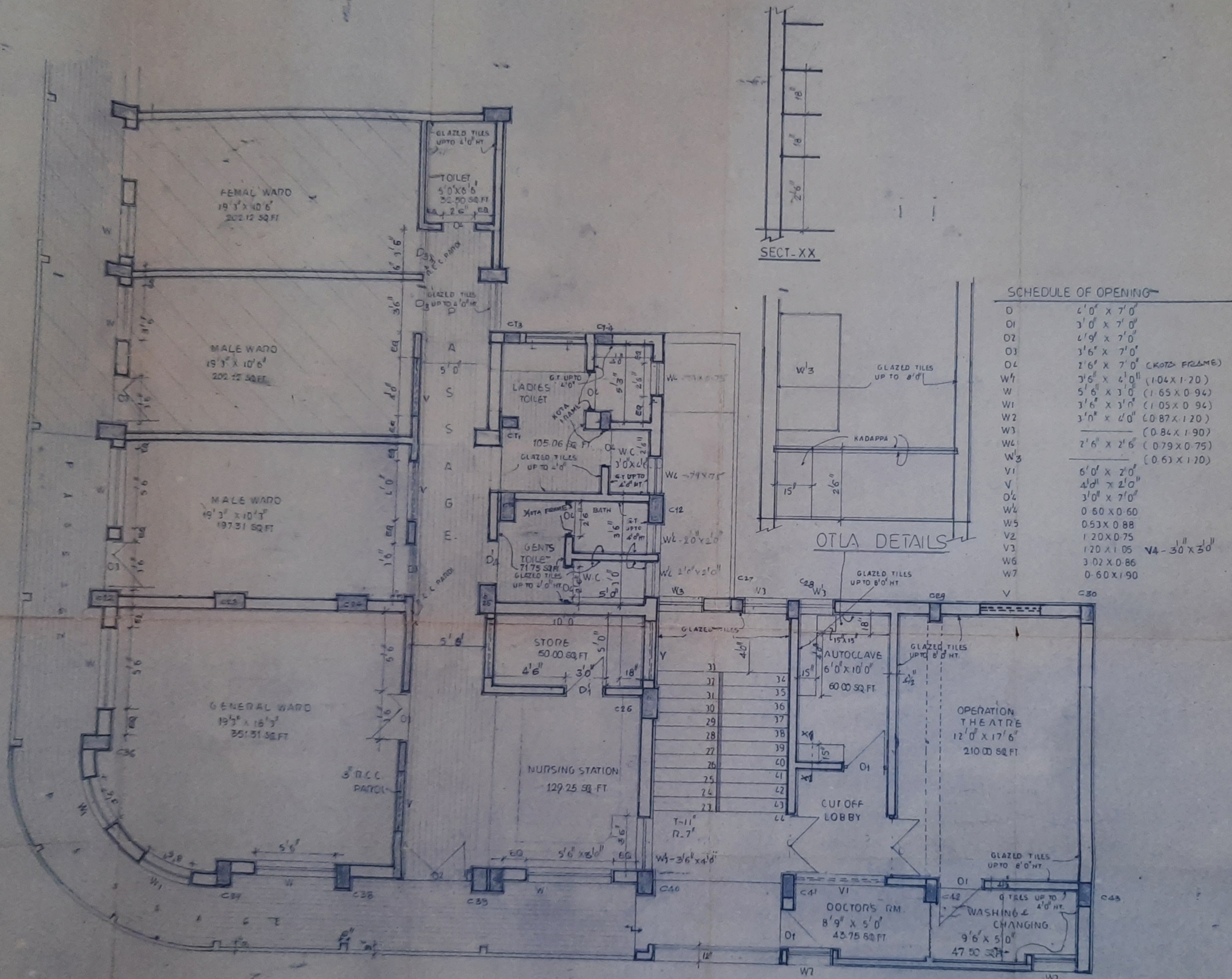
SECOND FLOOR PLAN TOTAL BUILT UP AREA INCLUDING PASSAGE - 3102.50 SQ FT HOMEOPATHIC COLLEGE
